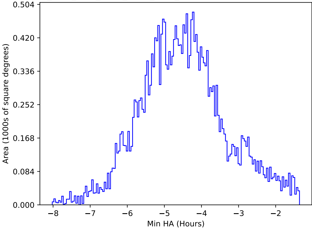
ddf_acor_sf10_lsf20_lsr10_v3.4_10yrs All sky all bands: Min HA
