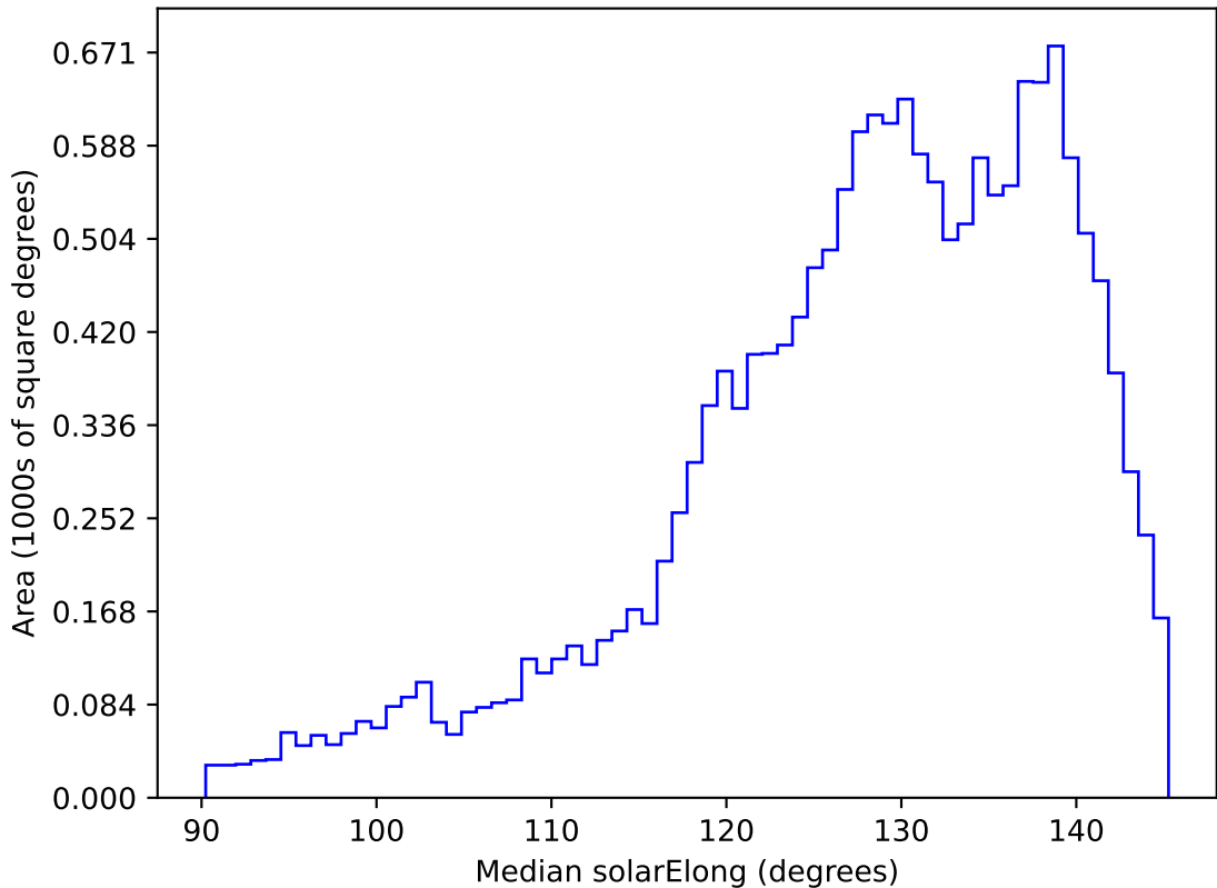
ddf_acor_sf10_lsf20_lsr10_v3.4_10yrs WFD z band: Median solarElong
