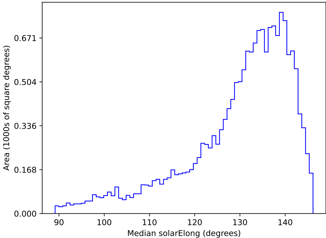
ddf_acor_sf10_lsf20_lsr10_v3.4_10yrs WFD y band: Median solarElong
