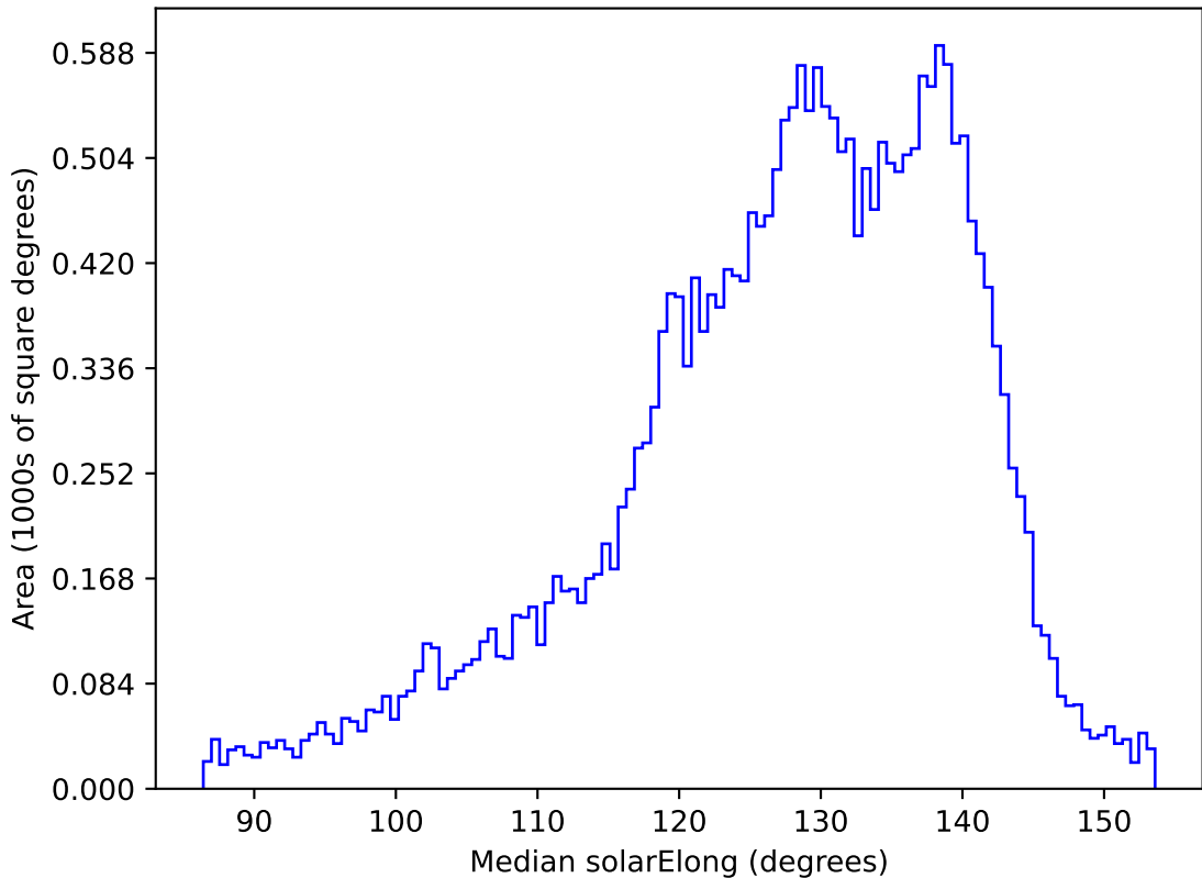
ddf_acor_sf10_lsf20_lsr10_v3.4_10yrs All sky z band: Median solarElong
