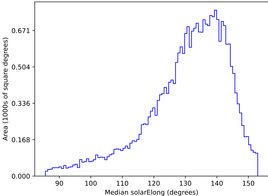
ddf_acor_sf10_lsf20_lsr10_v3.4_10yrs All sky r band: Median solarElong
