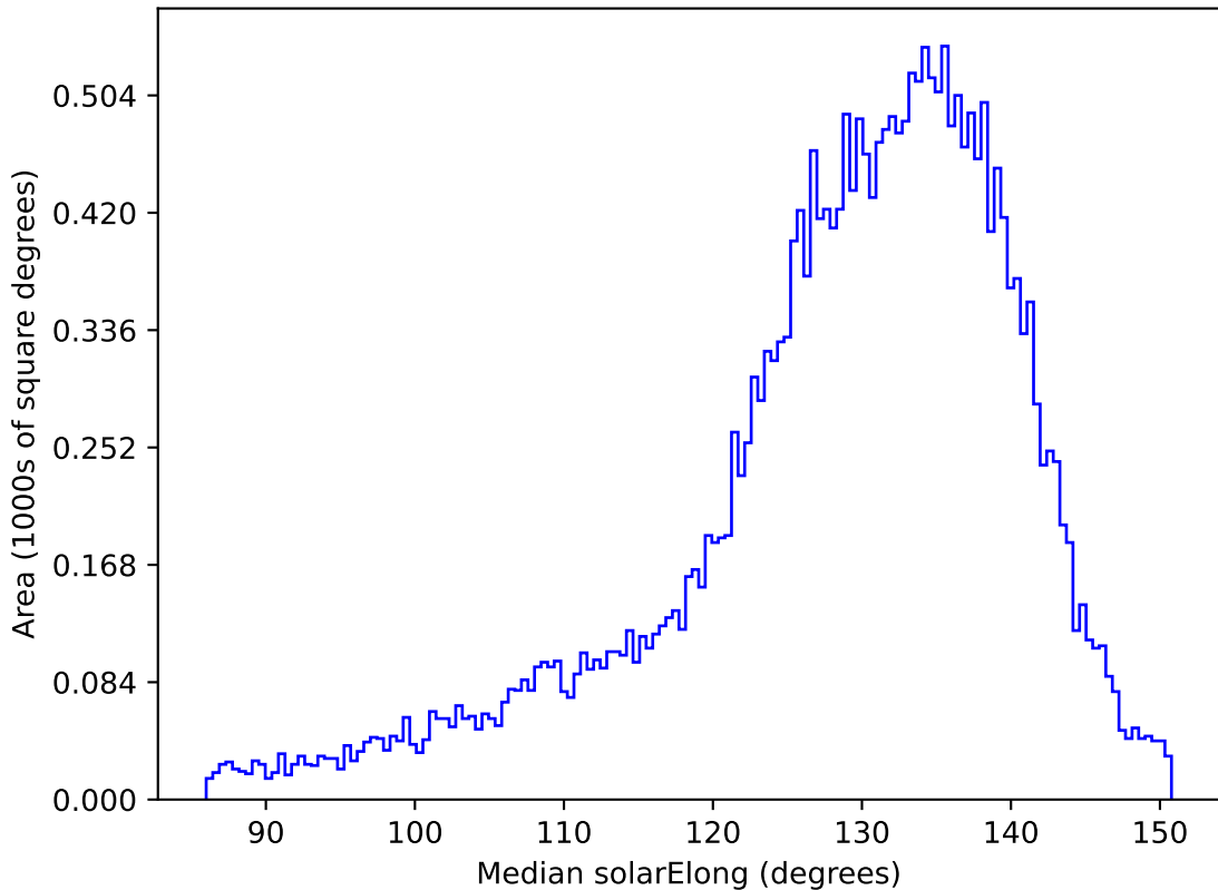
ddf_acor_sf10_lsf20_lsr10_v3.4_10yrs All sky i band: Median solarElong
