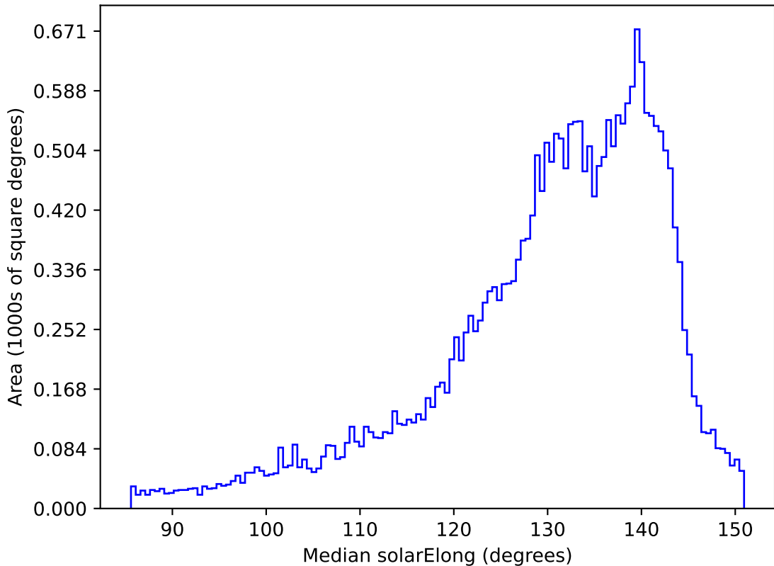
ddf_acor_sf10_lsf20_lsr10_v3.4_10yrs All sky all bands: Median solarElong
