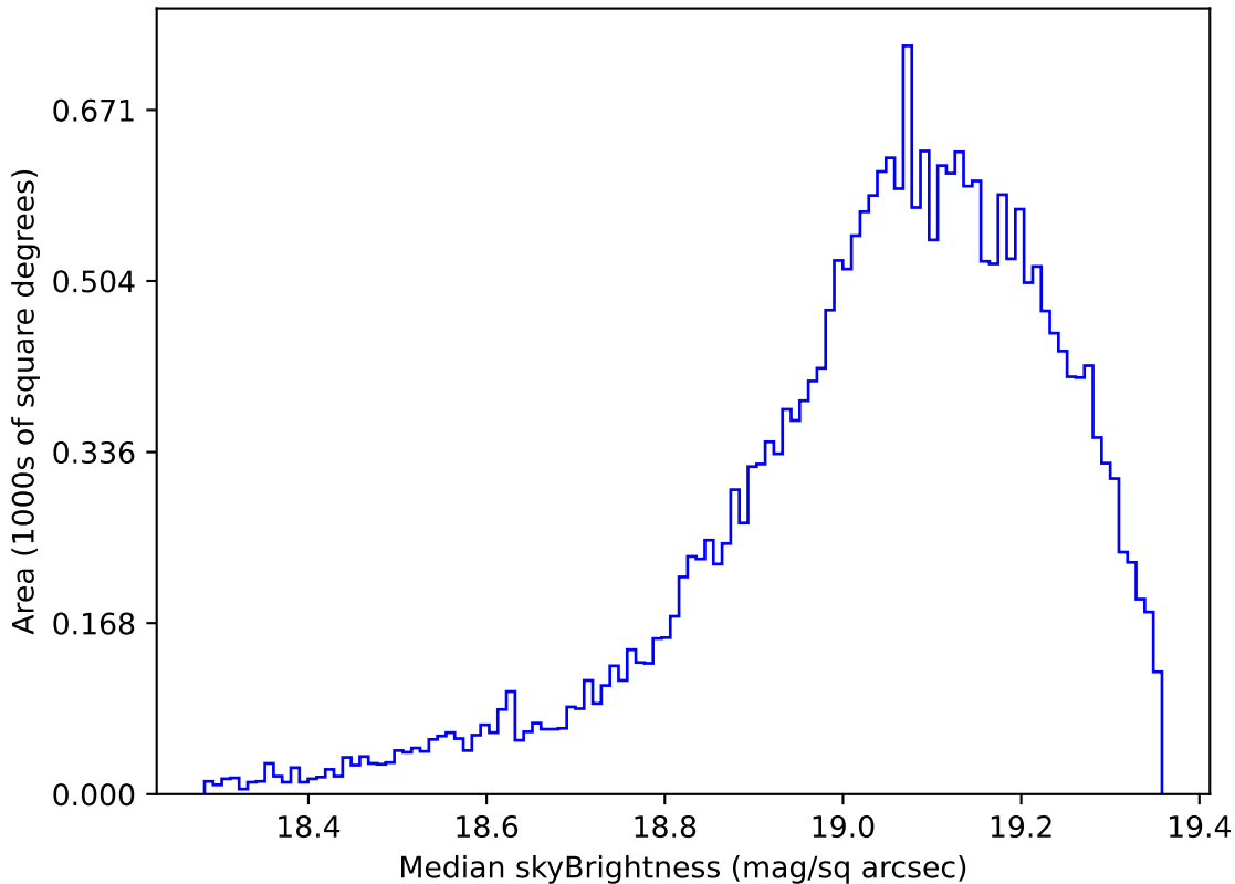
ddf_acor_sf10_lsf20_lsr10_v3.4_10yrs Yr 1 z band: Median skyBrightness
