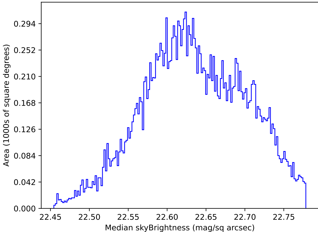
ddf_acor_sf10_lsf20_lsr10_v3.4_10yrs Yr 1 u band: Median skyBrightness
