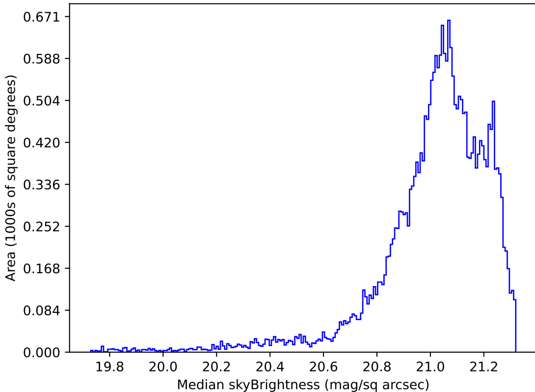
ddf_acor_sf10_lsf20_lsr10_v3.4_10yrs Yr 1 r band: Median skyBrightness
