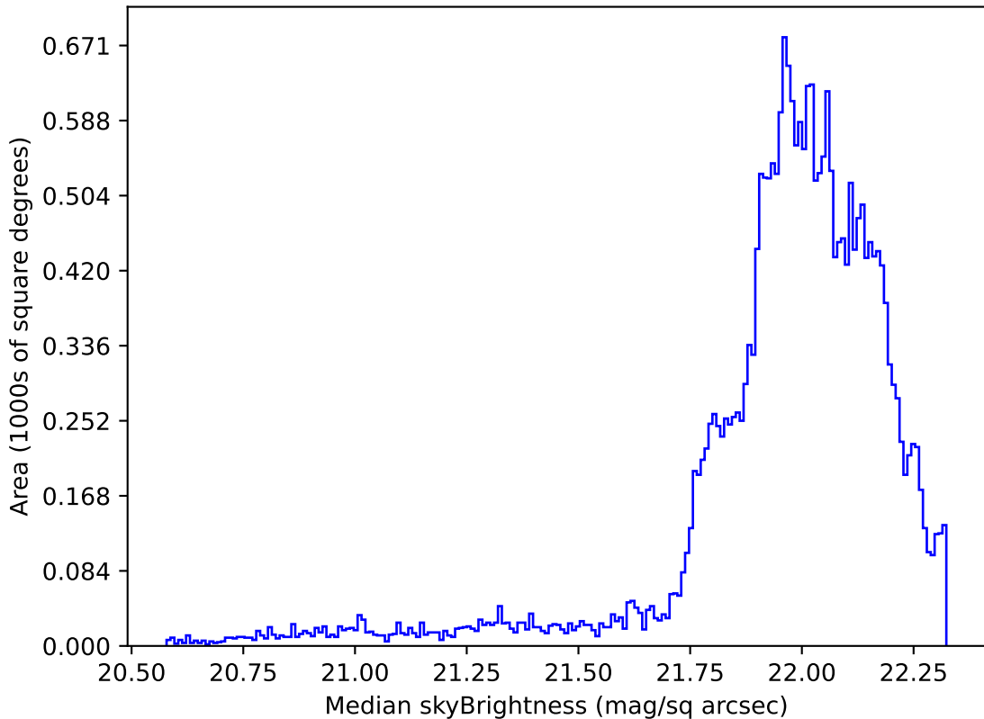
ddf_acor_sf10_lsf20_lsr10_v3.4_10yrs Yr 1 g band: Median skyBrightness
