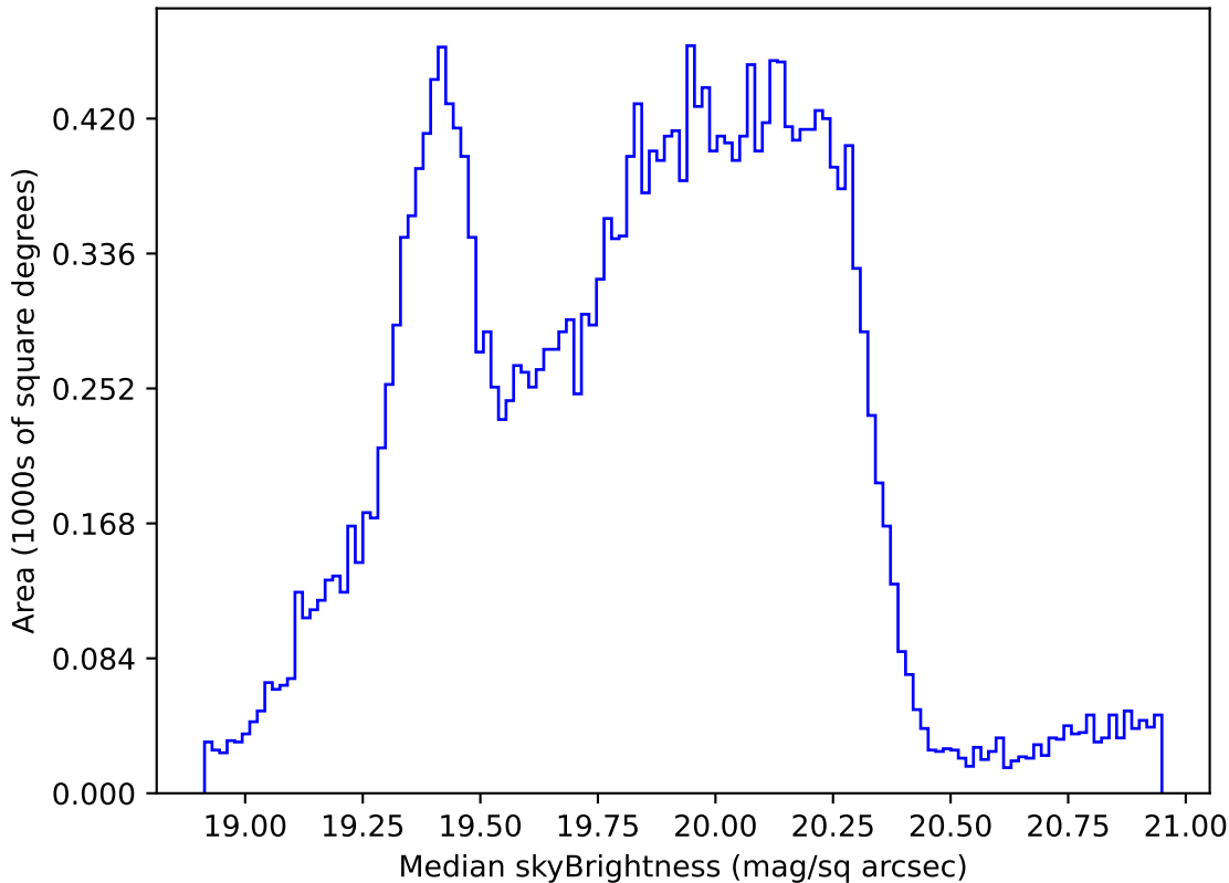
ddf_acor_sf10_lsf20_lsr10_v3.4_10yrs Yr 1 all bands: Median skyBrightness
