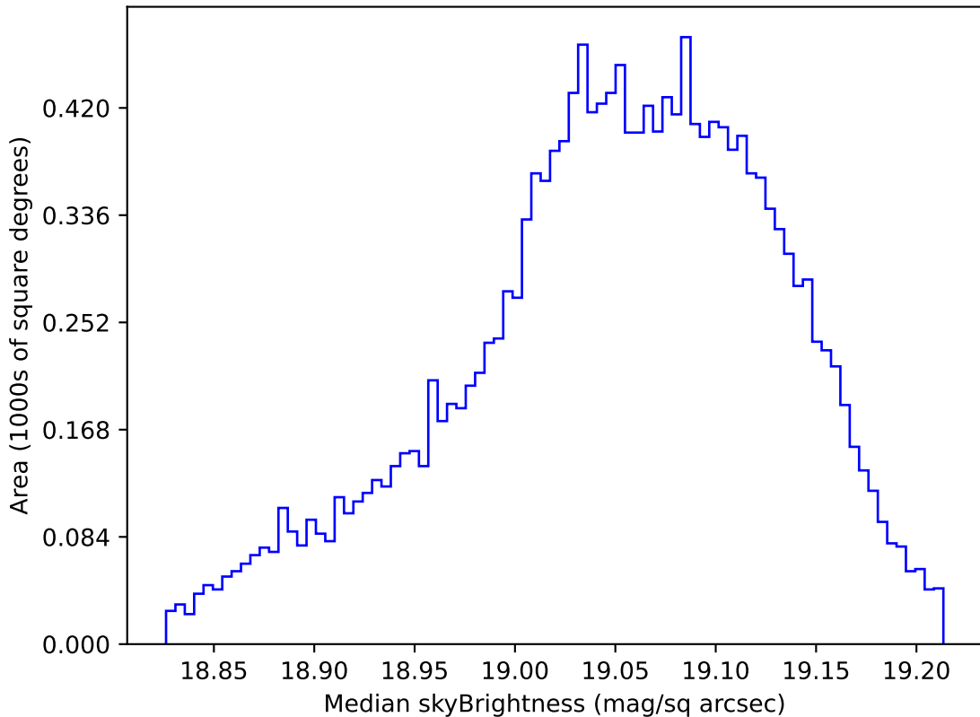
ddf_acor_sf10_lsf20_lsr10_v3.4_10yrs WFD z band: Median skyBrightness
