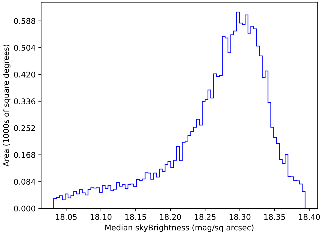
ddf_acor_sf10_lsf20_lsr10_v3.4_10yrs WFD y band: Median skyBrightness
