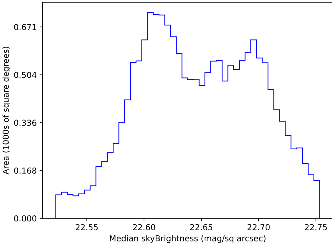
ddf_acor_sf10_lsf20_lsr10_v3.4_10yrs WFD u band: Median skyBrightness
