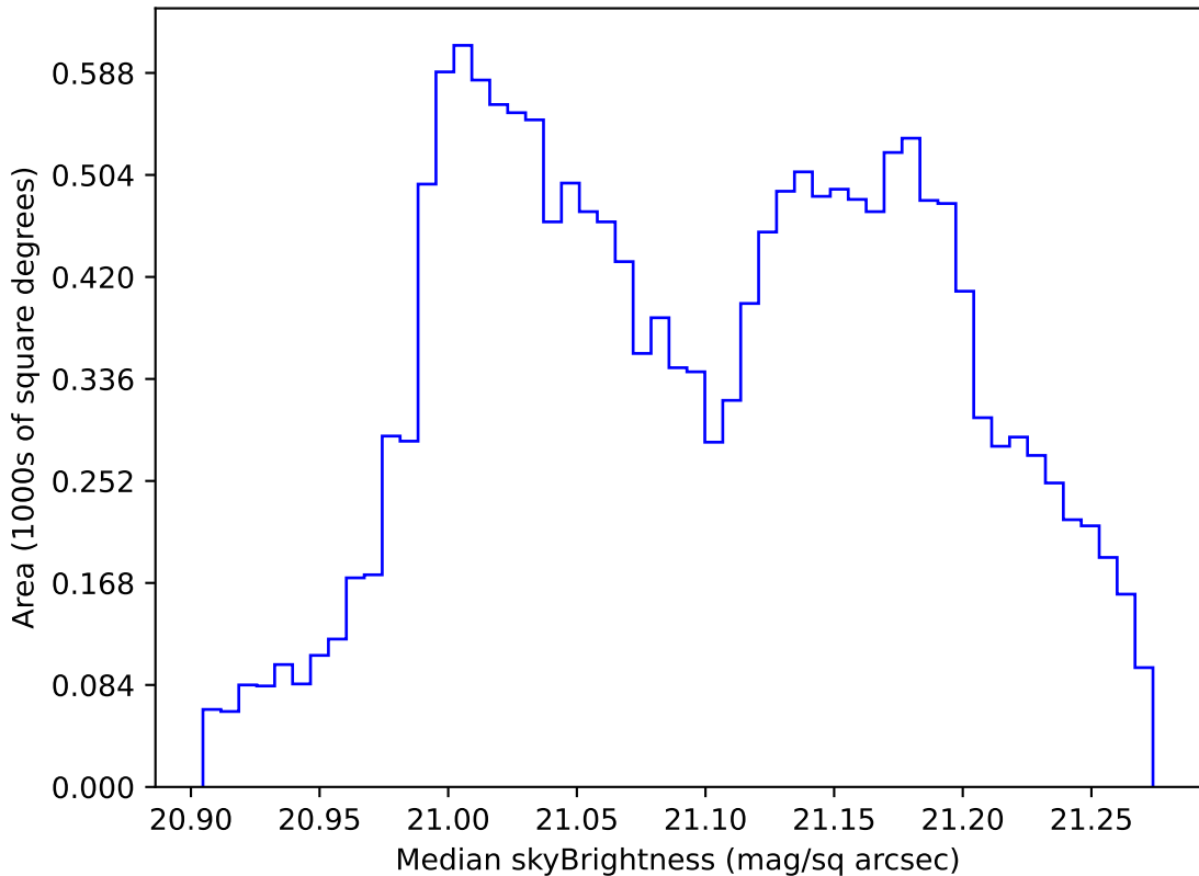
ddf_acor_sf10_lsf20_lsr10_v3.4_10yrs WFD r band: Median skyBrightness
