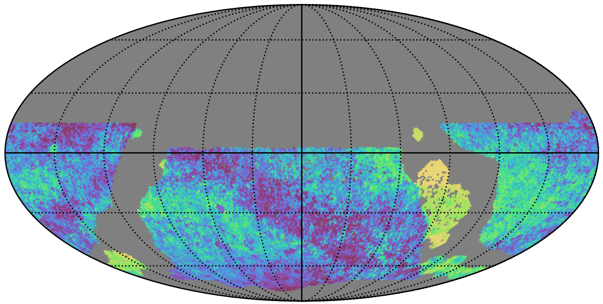
ddf_acor_sf10_lsf20_lsr10_v3.4_10yrs WFD all bands: Median skyBrightness
