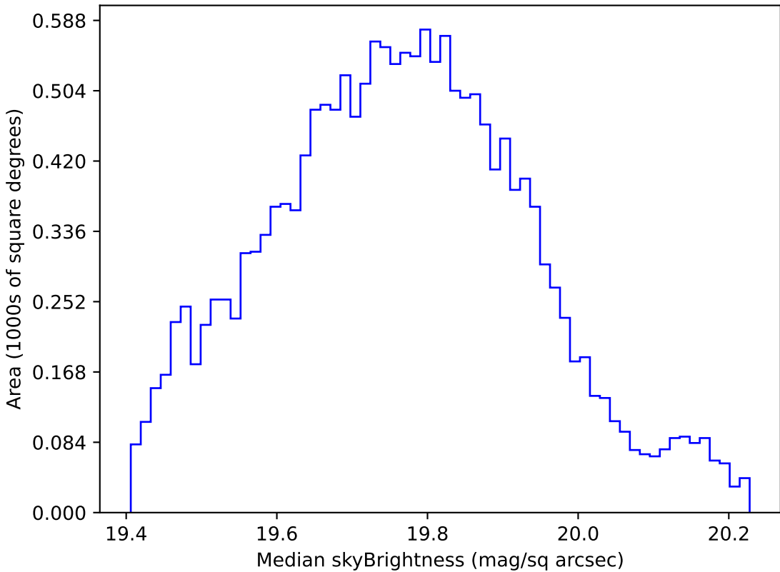
ddf_acor_sf10_lsf20_lsr10_v3.4_10yrs WFD all bands: Median skyBrightness
