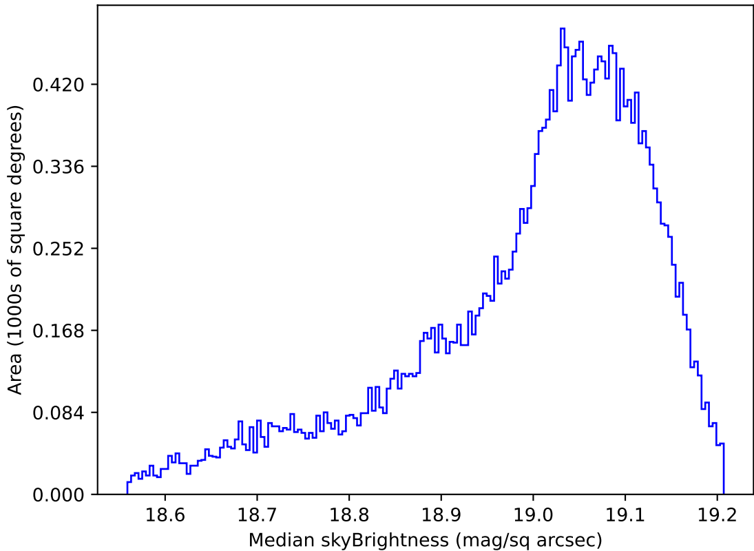
ddf_acor_sf10_lsf20_lsr10_v3.4_10yrs All sky z band: Median skyBrightness
