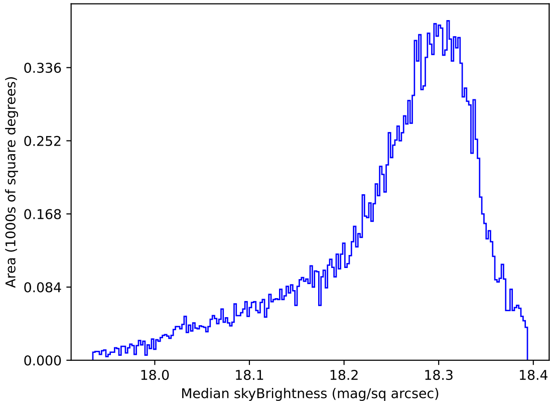
ddf_acor_sf10_lsf20_lsr10_v3.4_10yrs All sky y band: Median skyBrightness
