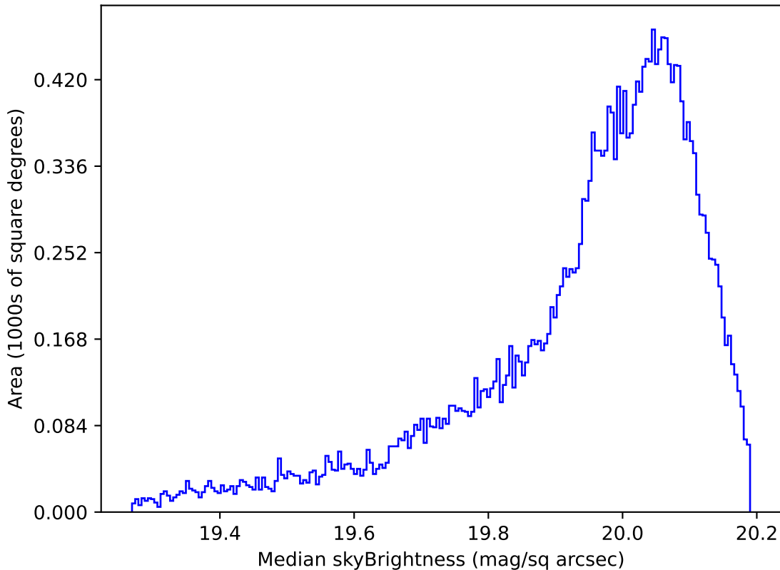
ddf_acor_sf10_lsf20_lsr10_v3.4_10yrs All sky i band: Median skyBrightness
