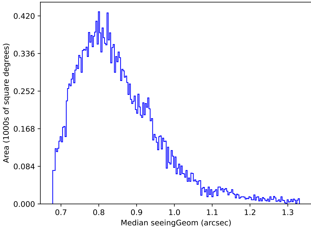
ddf_acor_sf10_lsf20_lsr10_v3.4_10yrs Yr 1 z band: Median seeingGeom
