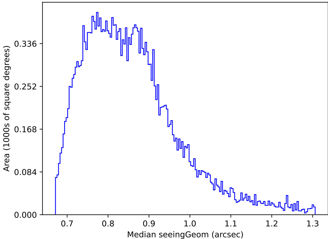
ddf_acor_sf10_lsf20_lsr10_v3.4_10yrs Yr 1 r band: Median seeingGeom
