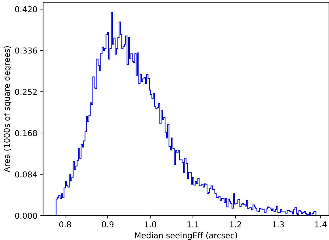
ddf_acor_sf10_lsf20_lsr10_v3.4_10yrs Yr 1 y band: Median seeingEff
