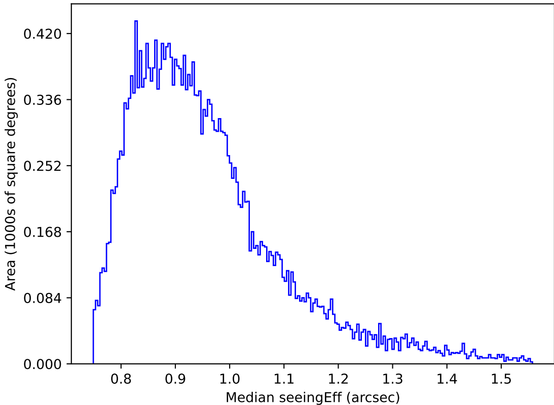
ddf_acor_sf10_lsf20_lsr10_v3.4_10yrs Yr 1 i band: Median seeingEff
