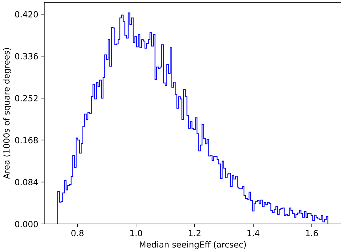
ddf_acor_sf10_lsf20_lsr10_v3.4_10yrs Yr 1 g band: Median seeingEff
