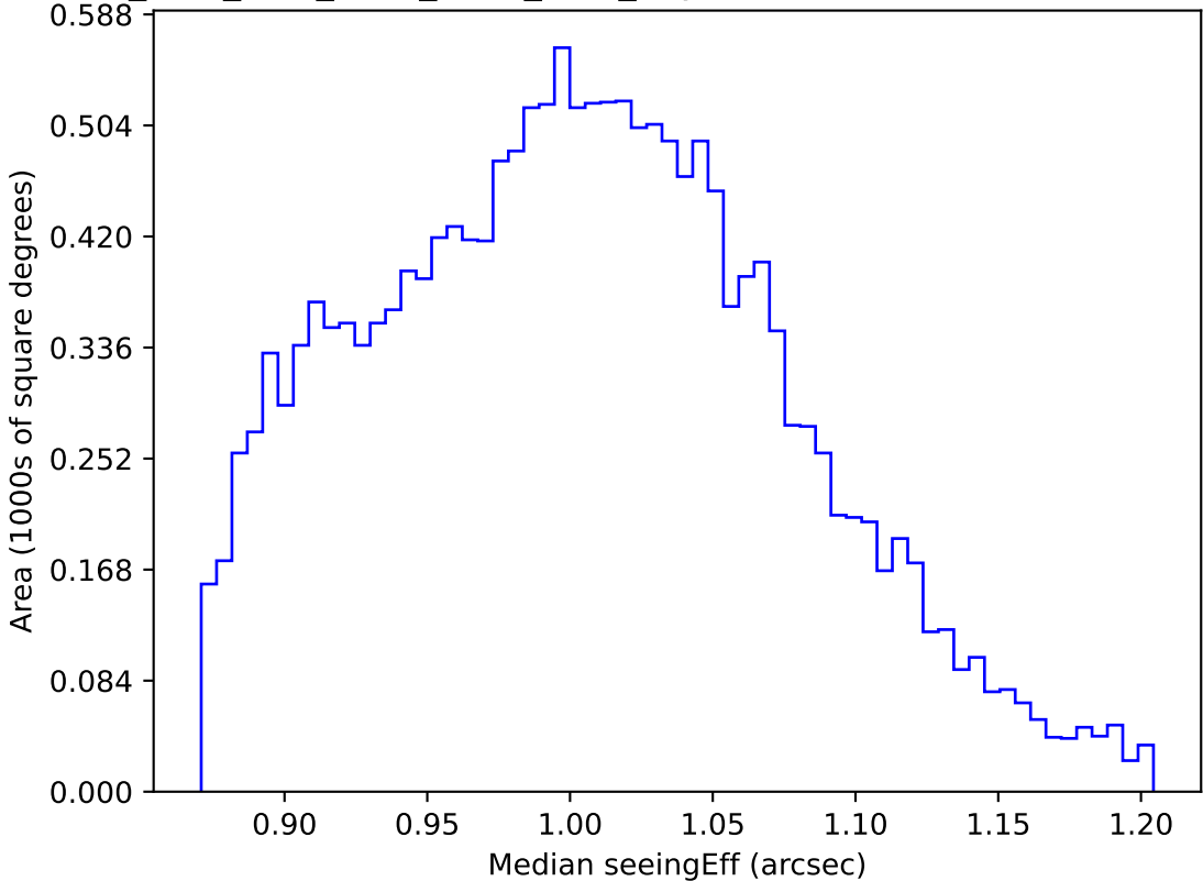
ddf_acor_sf10_lsf20_lsr10_v3.4_10yrs WFD z band: Median seeingEff
