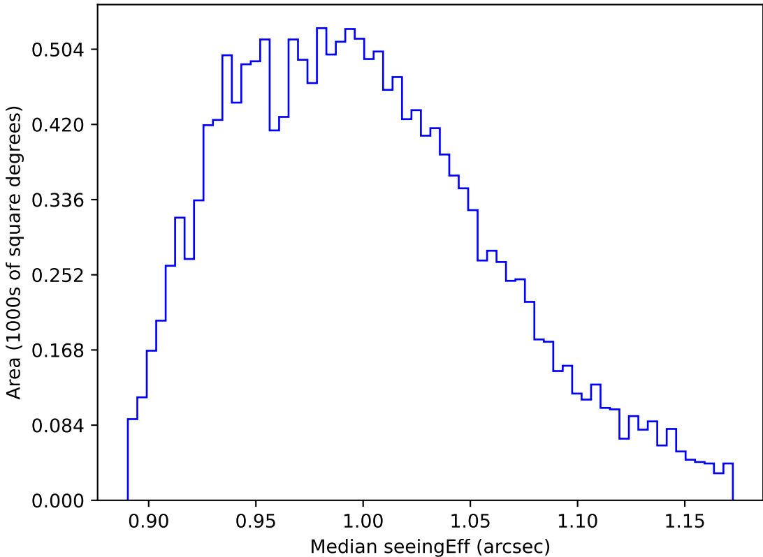
ddf_acor_sf10_lsf20_lsr10_v3.4_10yrs WFD y band: Median seeingEff
