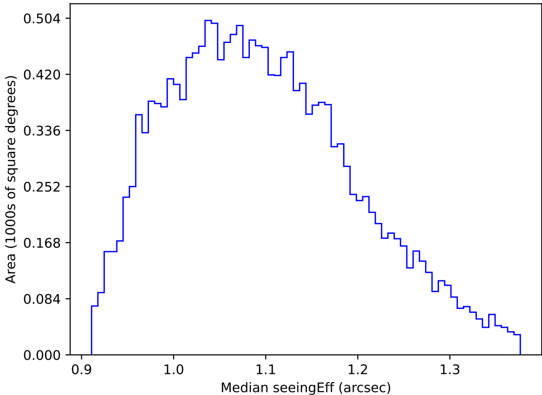
ddf_acor_sf10_lsf20_lsr10_v3.4_10yrs WFD g band: Median seeingEff
