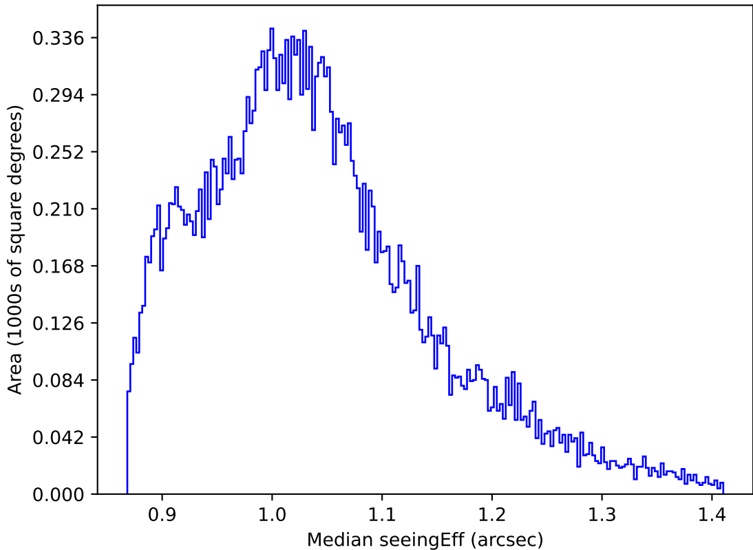
ddf_acor_sf10_lsf20_lsr10_v3.4_10yrs All sky z band: Median seeingEff
