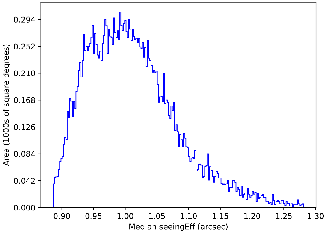
ddf_acor_sf10_lsf20_lsr10_v3.4_10yrs All sky y band: Median seeingEff
