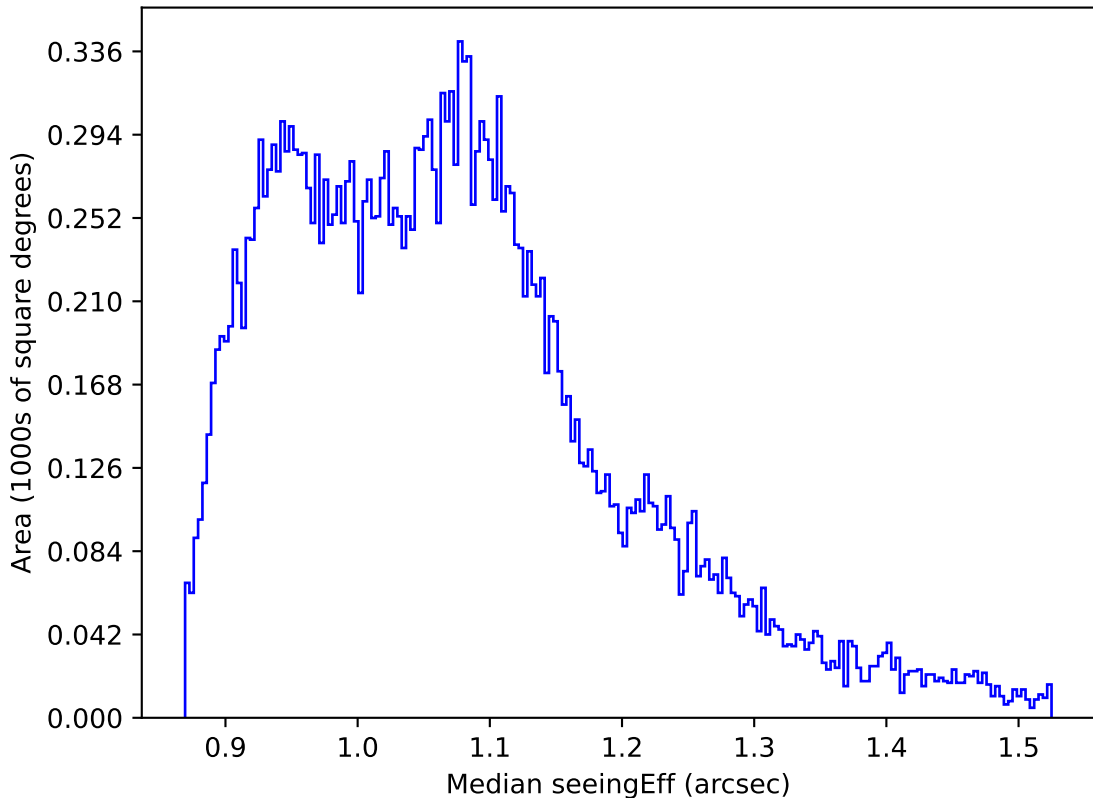
ddf_acor_sf10_lsf20_lsr10_v3.4_10yrs All sky r band: Median seeingEff
