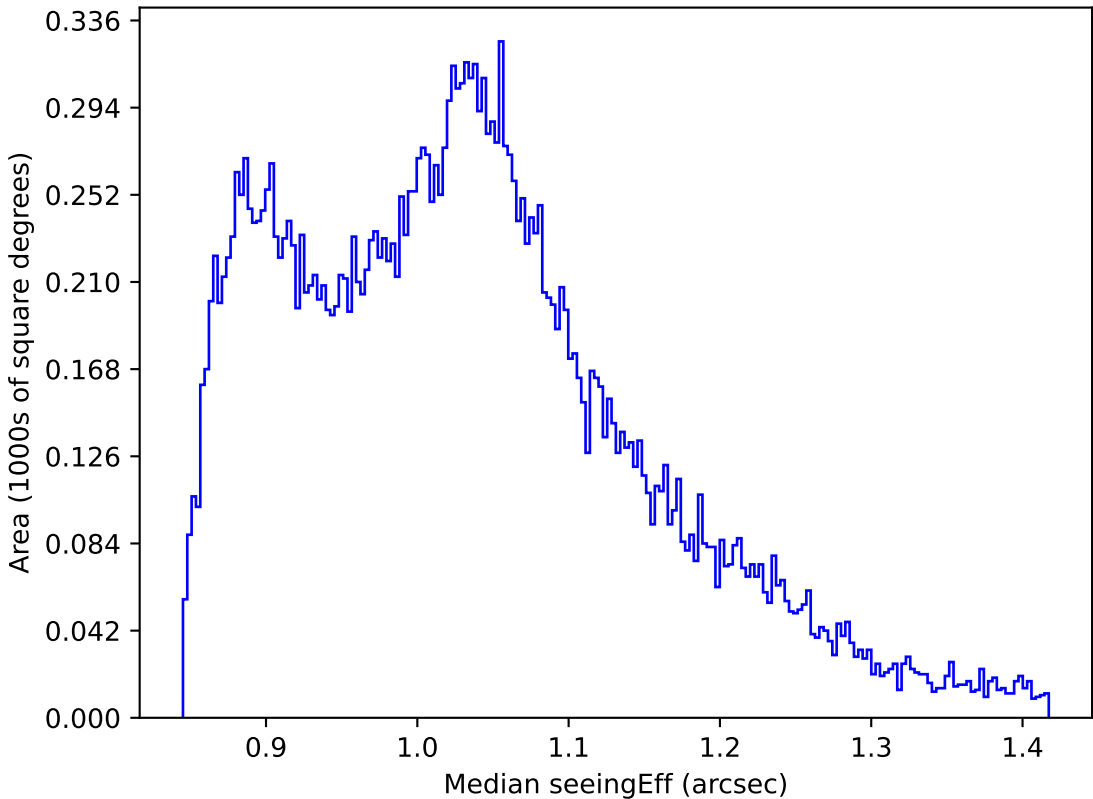
ddf_acor_sf10_lsf20_lsr10_v3.4_10yrs All sky i band: Median seeingEff
