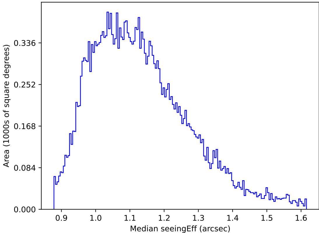
ddf_acor_sf10_lsf20_lsr10_v3.4_10yrs All sky g band: Median seeingEff
