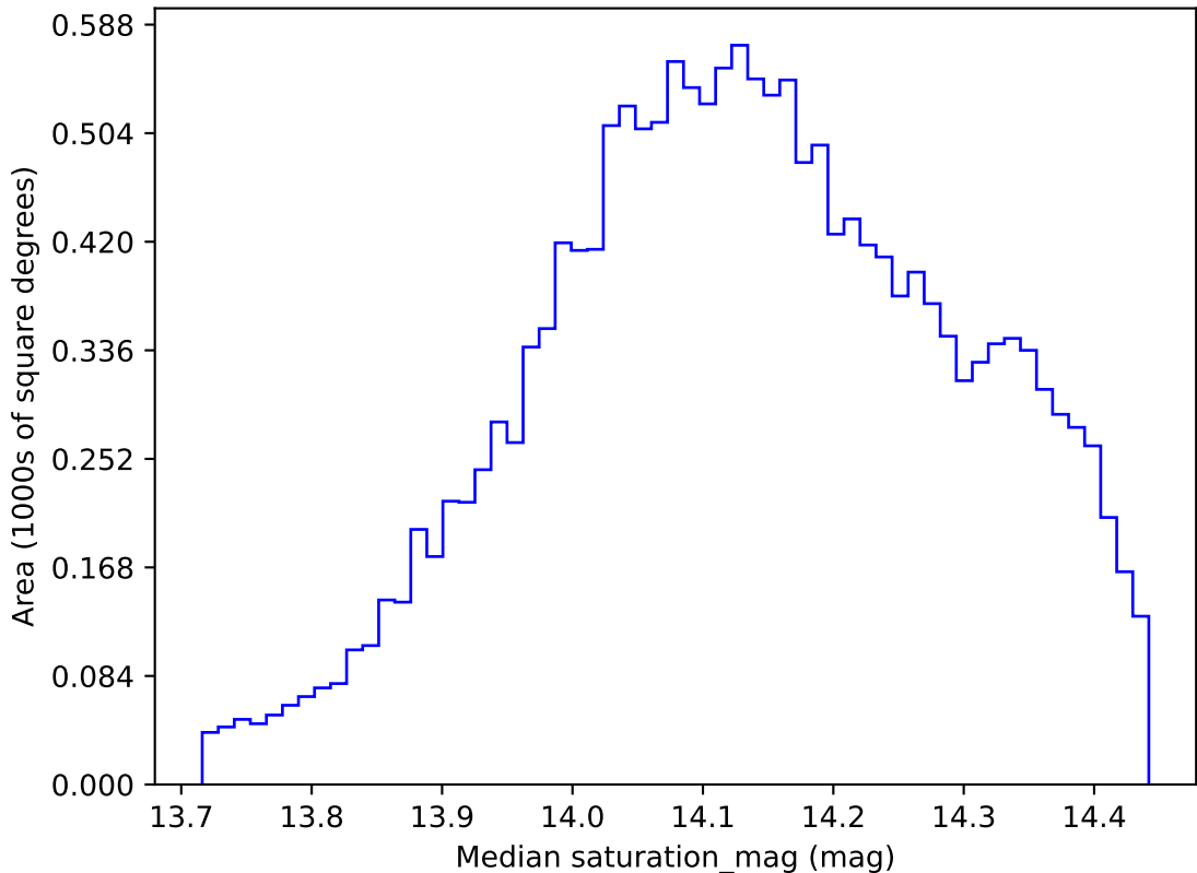
ddf_acor_sf10_lsf20_lsr10_v3.4_10yrs WFD z band: Median saturation_mag
