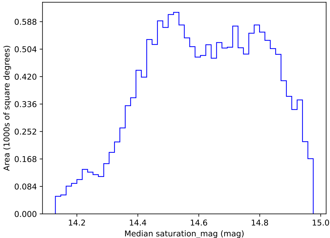
ddf_acor_sf10_lsf20_lsr10_v3.4_10yrs WFD r band: Median saturation_mag
