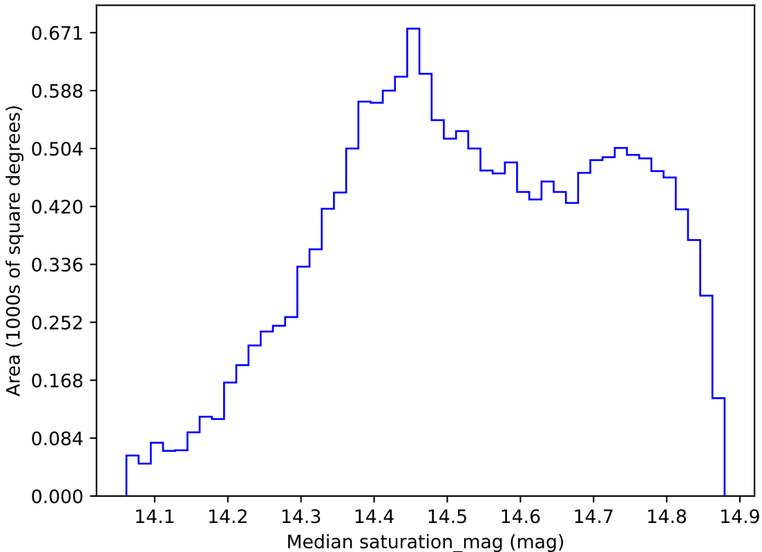
ddf_acor_sf10_lsf20_lsr10_v3.4_10yrs WFD i band: Median saturation_mag
