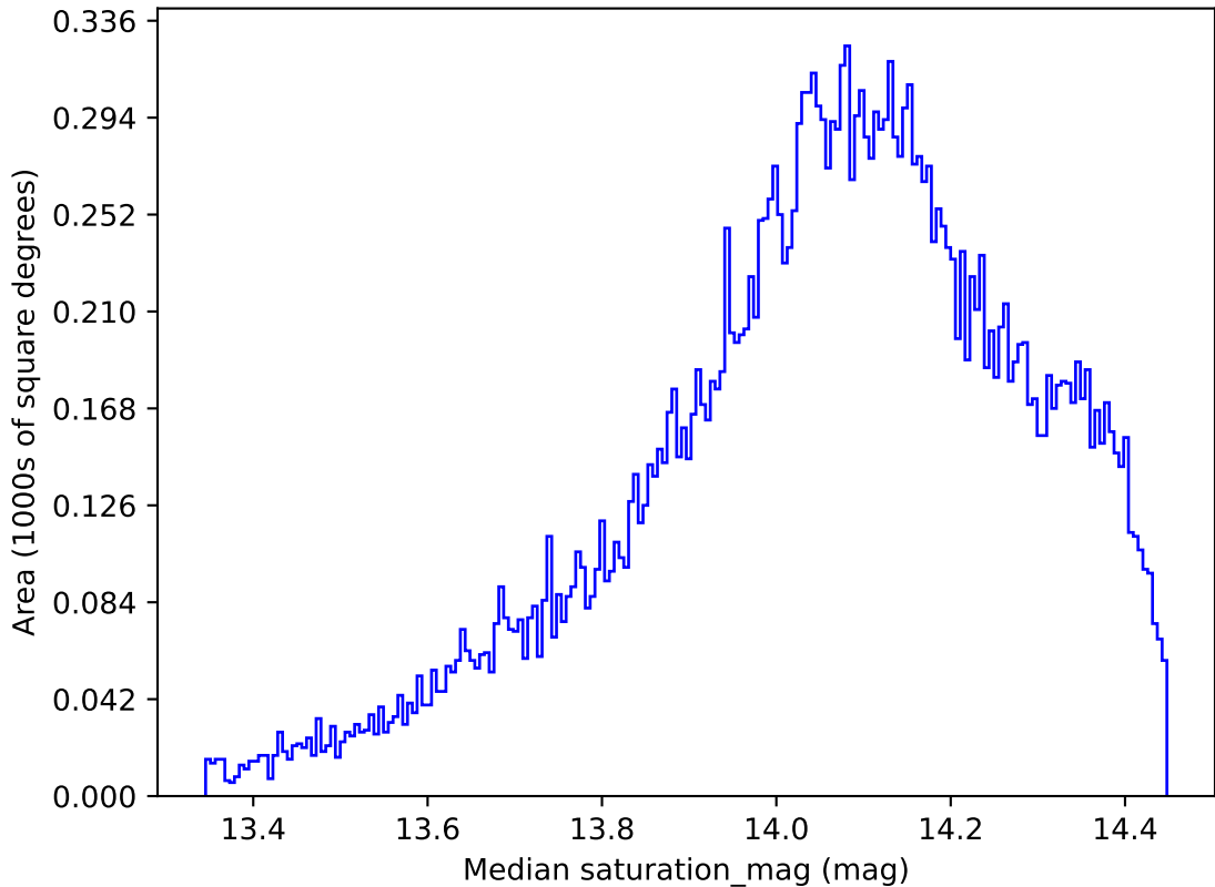
ddf_acor_sf10_lsf20_lsr10_v3.4_10yrs All sky z band: Median saturation_mag
