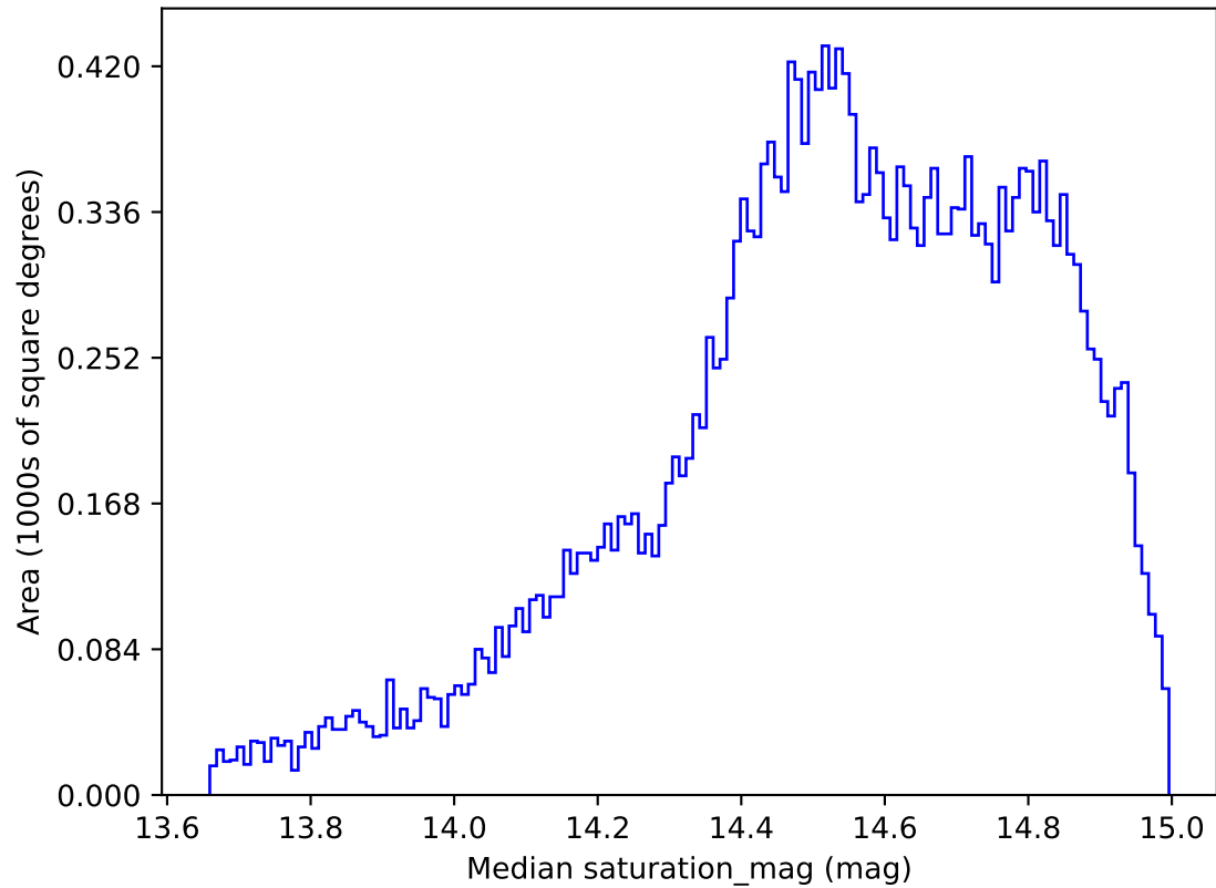
ddf_acor_sf10_lsf20_lsr10_v3.4_10yrs All sky r band: Median saturation_mag
