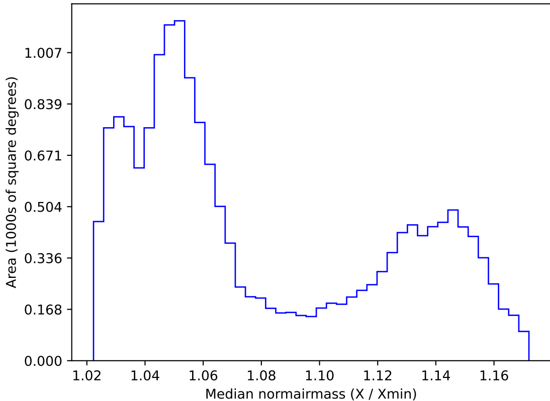
ddf_acor_sf10_lsf20_lsr10_v3.4_10yrs WFD all bands: Median normairmass
