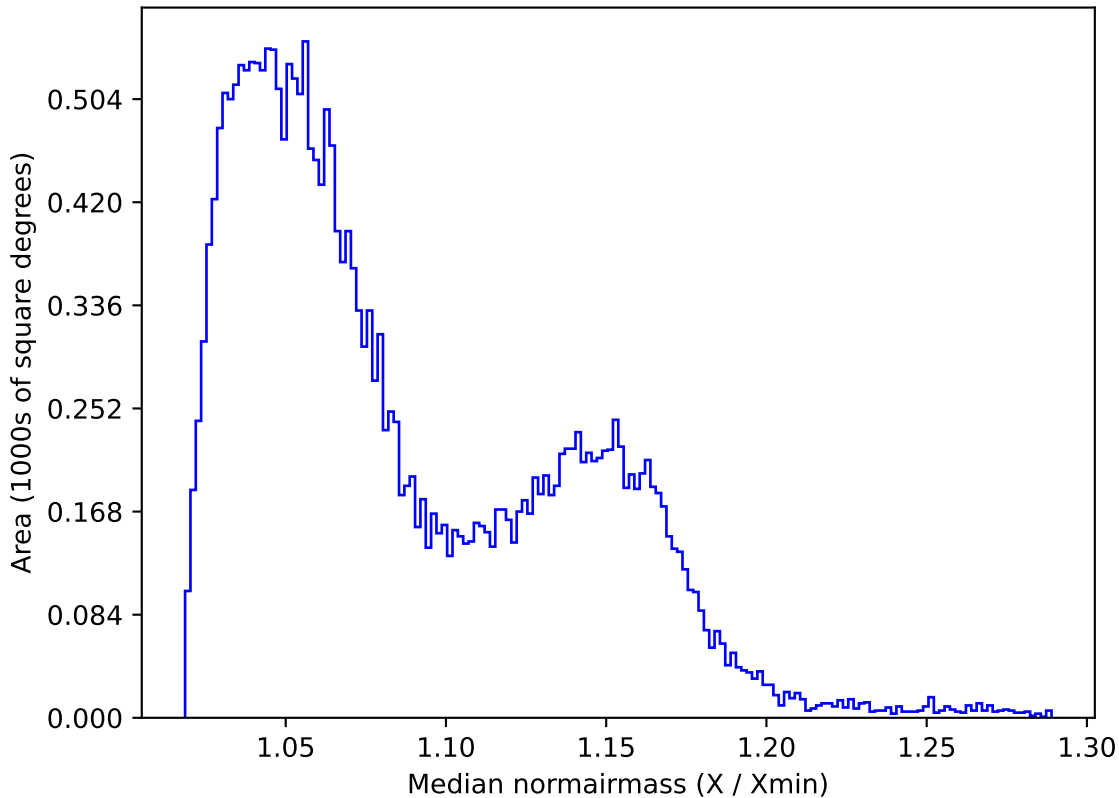
ddf_acor_sf10_ls20_lsr10_v3.4_10yrs All sky z band: Median normairmass
