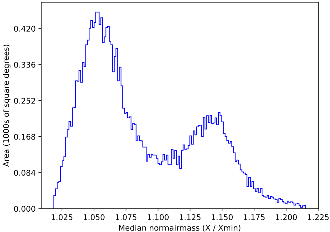
ddf_acor_sf10_ls20_lsr10_v3.4_10yrs All sky y band: Median normairmass
