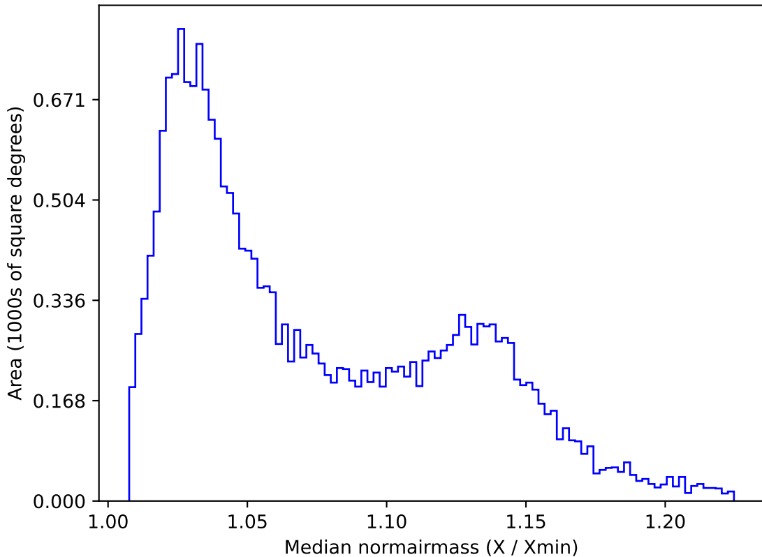
ddf_acor_sf10_lsf20_lsr10_v3.4_10yrs All sky u band: Median normairmass
