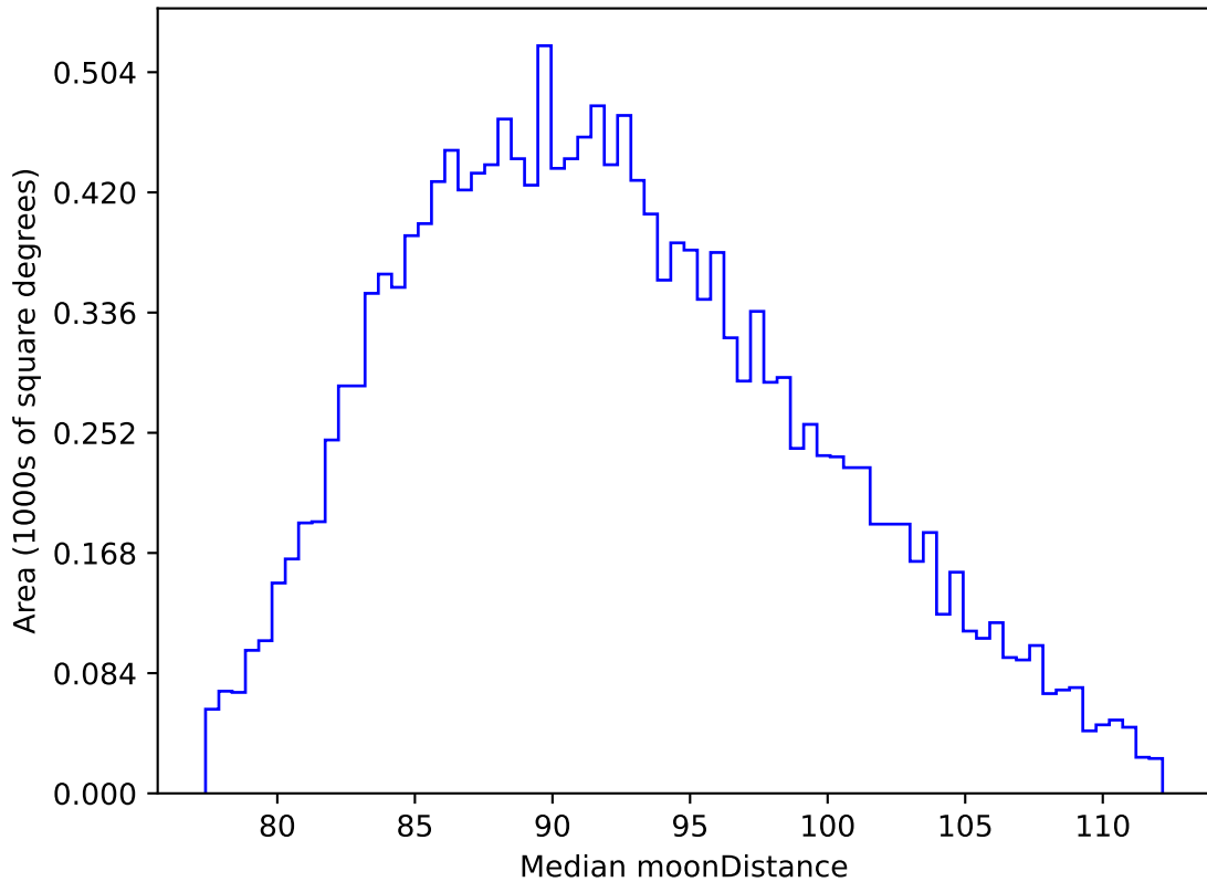
ddf_acor_sf10_lsf20_lsr10_v3.4_10yrs WFD i band: Median moonDistance
