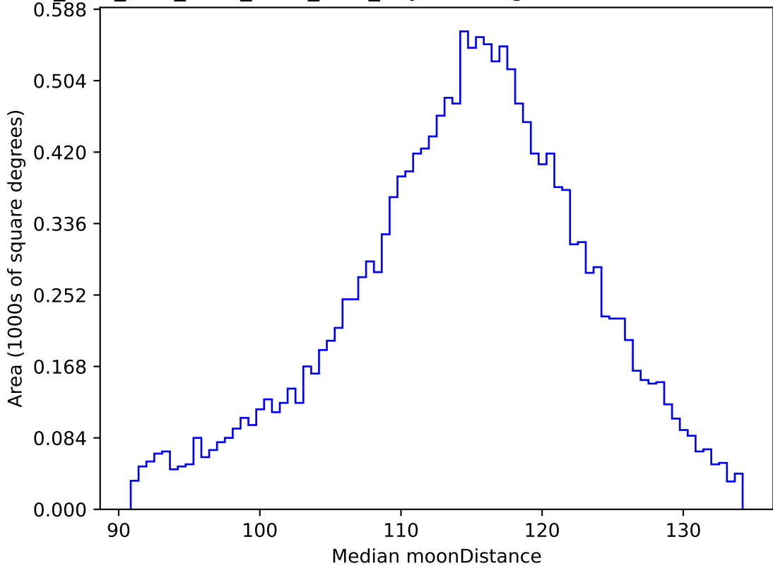
ddf_acor_sf10_lsf20_lsr10_v3.4_10yrs WFD g band: Median moonDistance
