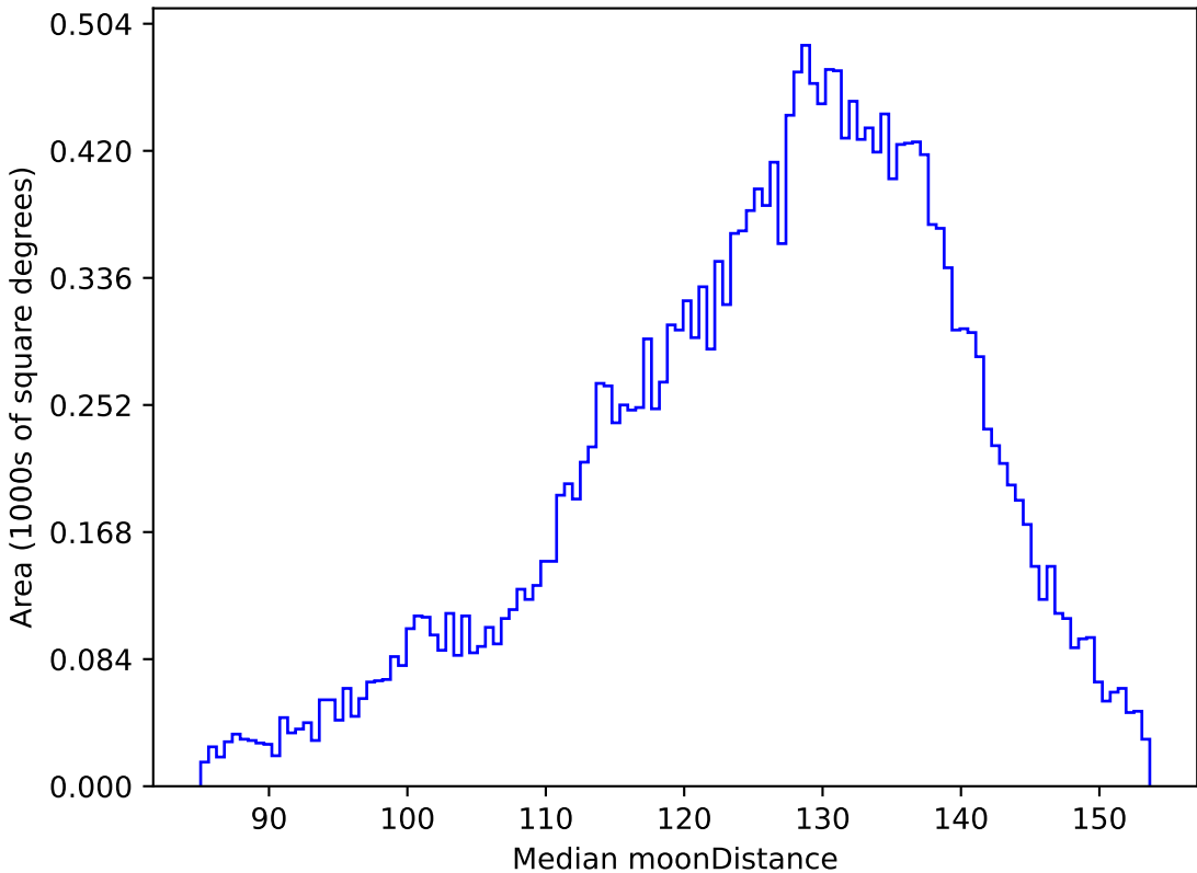
ddf_acor_sf10_lsf20_lsr10_v3.4_10yrs All sky u band: Median moonDistance
