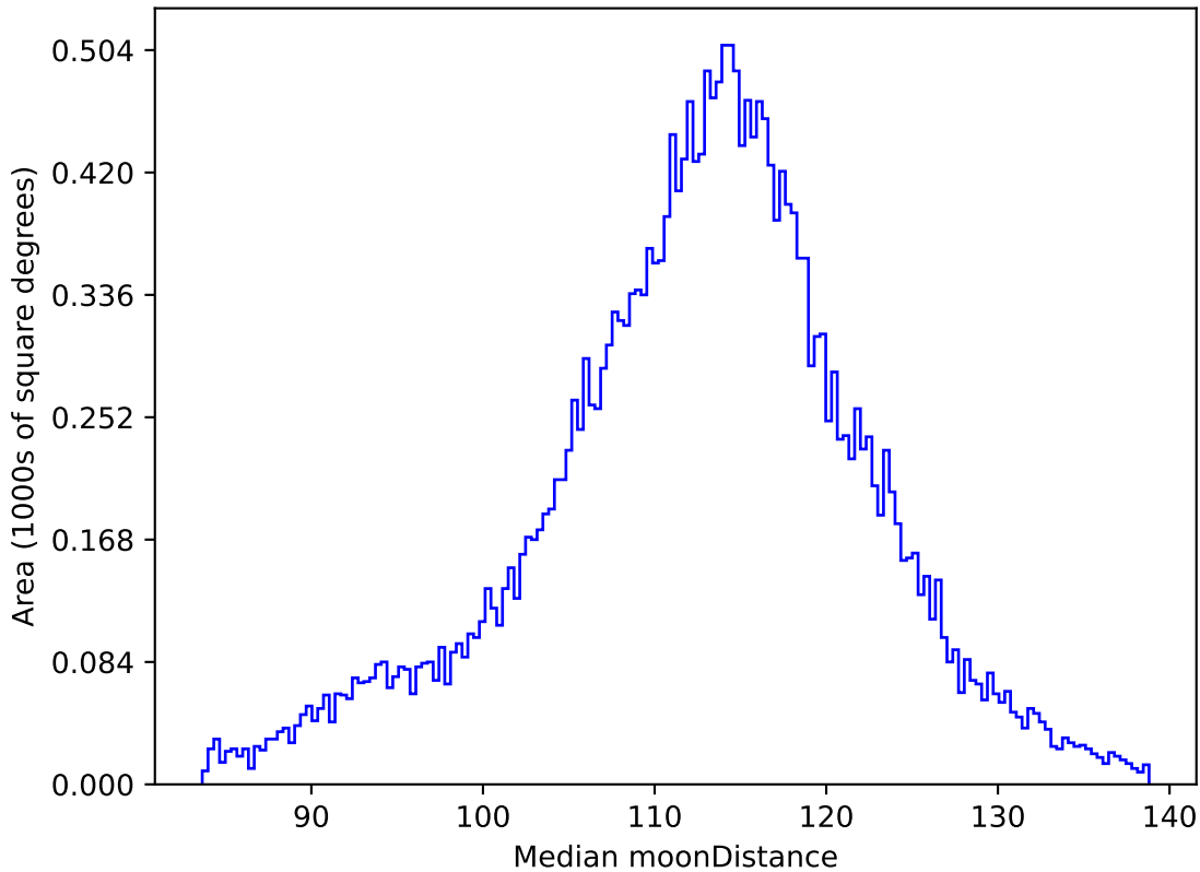
ddf_acor_sf10_lsf20_lsr10_v3.4_10yrs All sky r band: Median moonDistance
