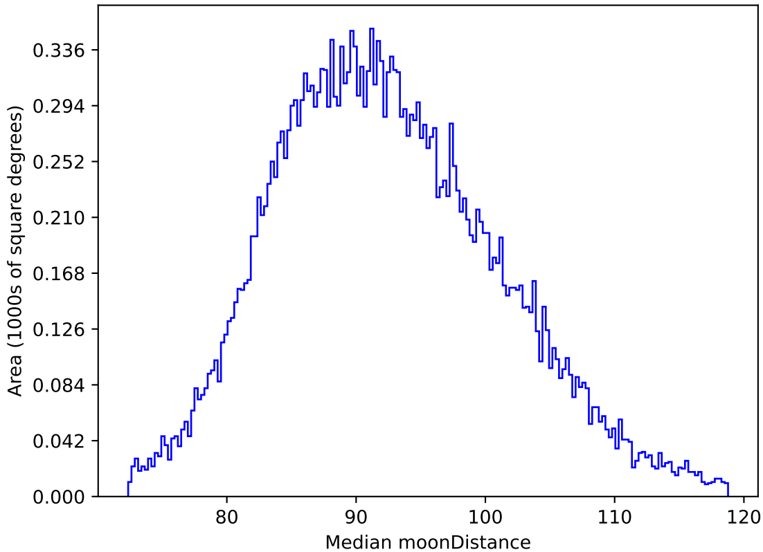
ddf_acor_sf10_lsf20_lsr10_v3.4_10yrs All sky i band: Median moonDistance
