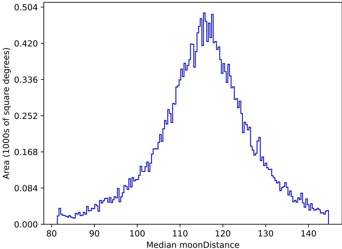
ddf_acor_sf10_lsf20_lsr10_v3.4_10yrs All sky g band: Median moonDistance
