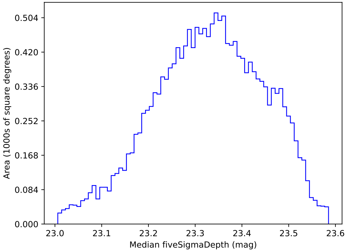
ddf_acor_sf10_lsf20_lsr10_v3.4_10yrs WFD all bands: Median fiveSigmaDepth
